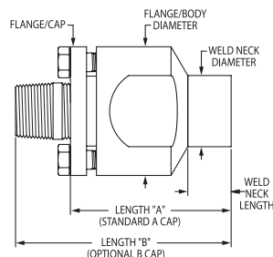
Flange Style Weld Neck Mount
