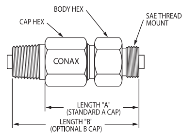
SAE Thread Mount
