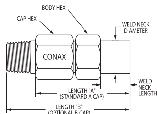
Weld Neck Mount
