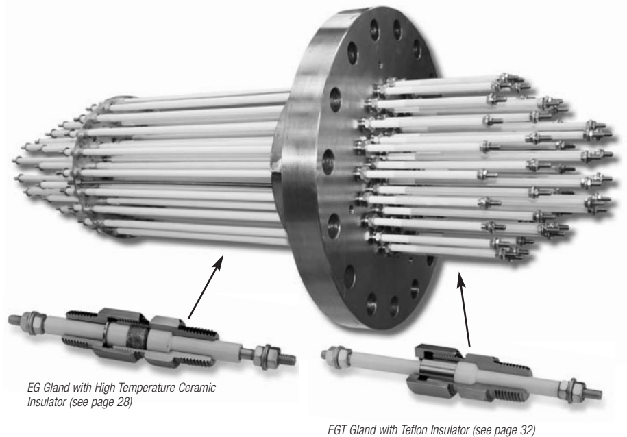
EGT Gland with Teflon Insulator (see page 32)
